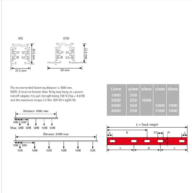
Track Dimensions and Loadings
